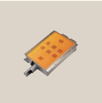
TRL DROP-IN INFRARED SEAR BURNER IRB-TRL BTU: 20,000
